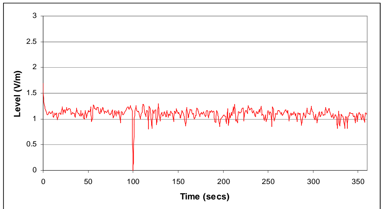
Electric field strengths recorded over 6 min period using 3 GHz probe at point of max NIR:
